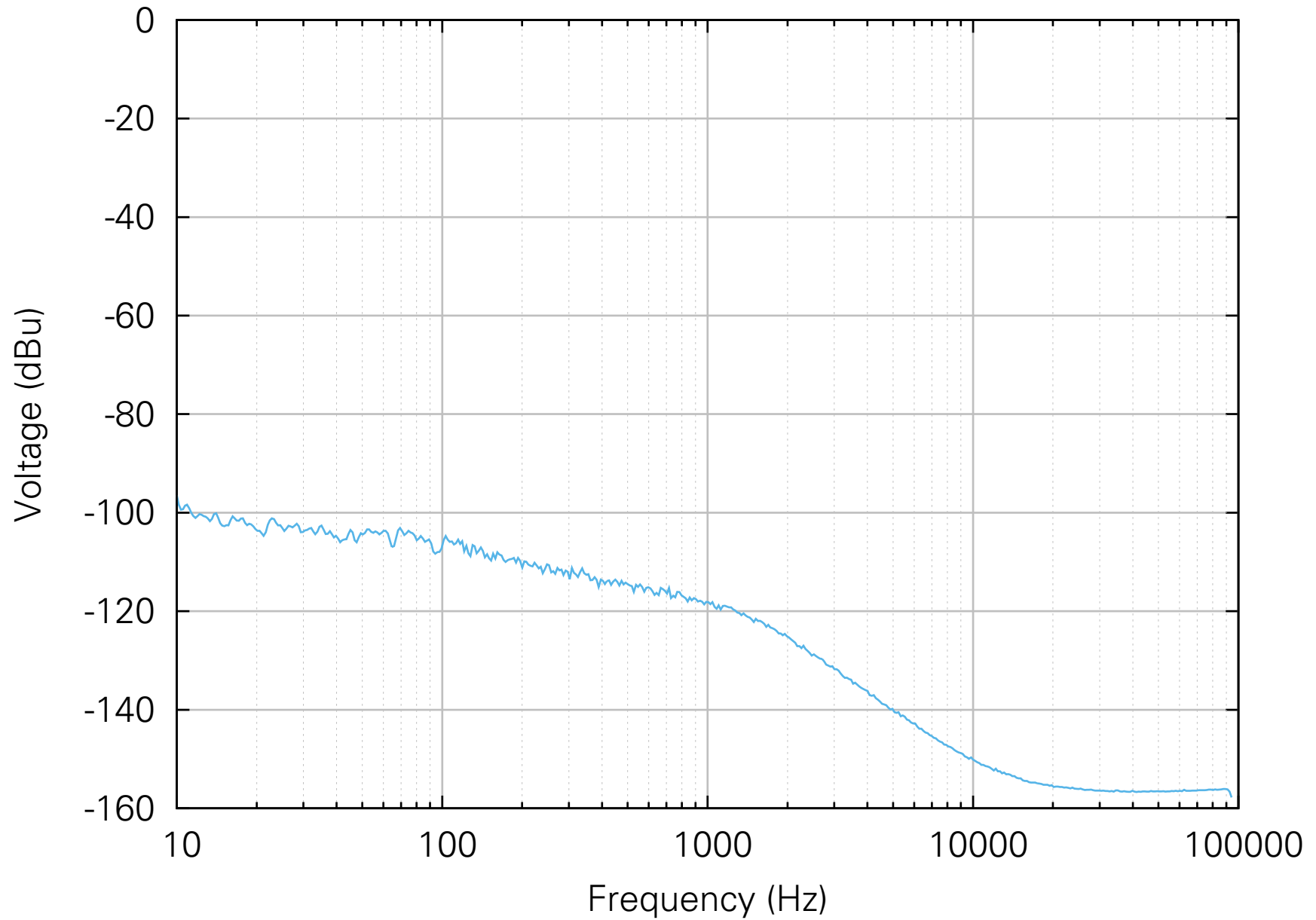
Output Voltage Noise (Idle Control Data and SOF)
