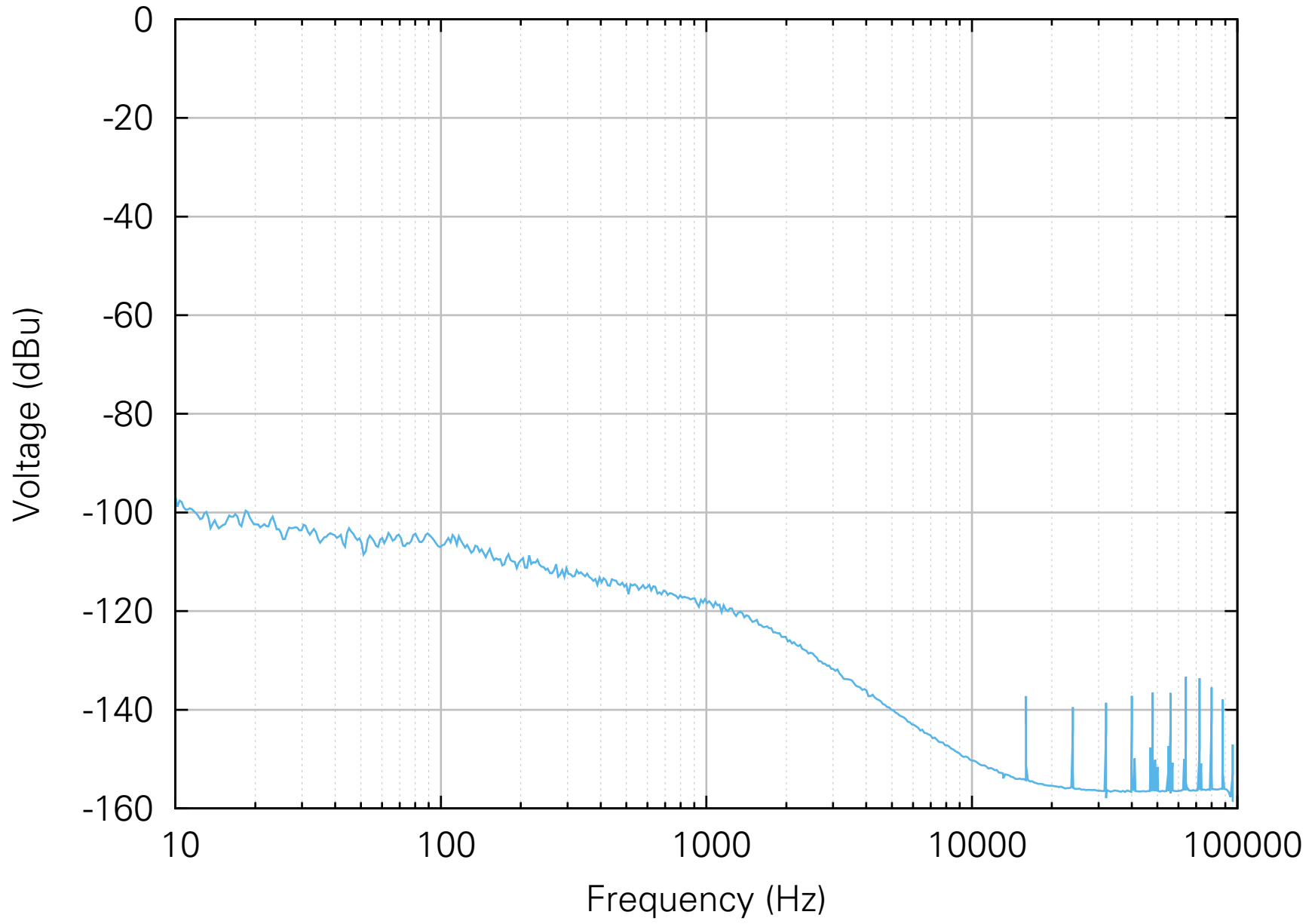
Output Voltage Noise (Full Downstream Utilization)
